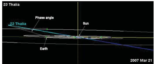
Figure 2. The inclined orbit of (23) Thalia at opposition.
